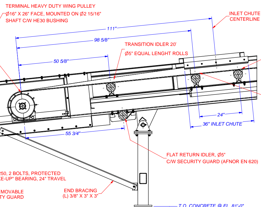
SECTION : TAIL DIMS & SPECS: TAIL DIMS & SPECS
