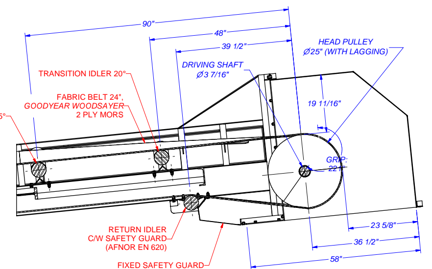
SECTION : HEAD DIMS & SPECS: HEAD DIMS & SPECS
