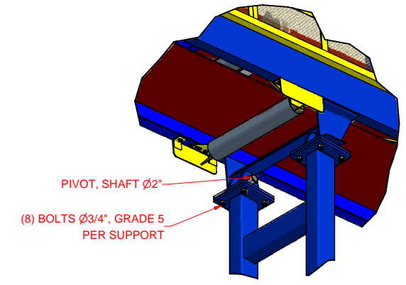
DETAIL : SUPPORT HOLDING
