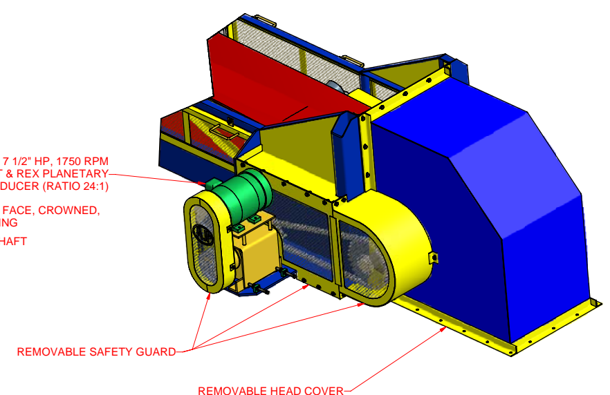
DETAIL E : HEAD COVER & SAFETY GUARDS
