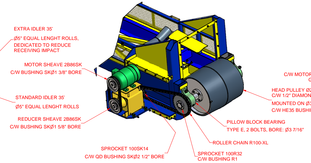
DETAIL : DRIVE SPECS
